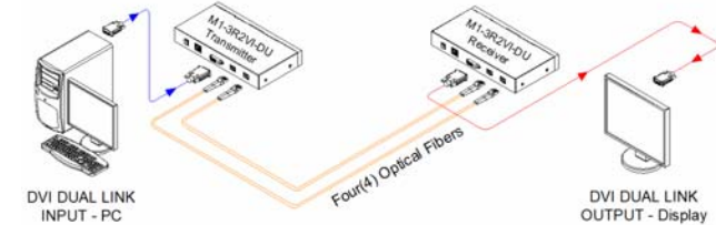
Figure 7 – Connection of 4 LC fiber cables
