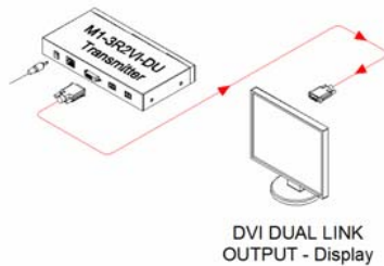
Figure 6 – Connection for Self-EDID programming
