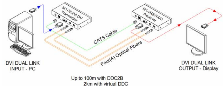
Figure 1 – Overall Optical dual link DVI Module
